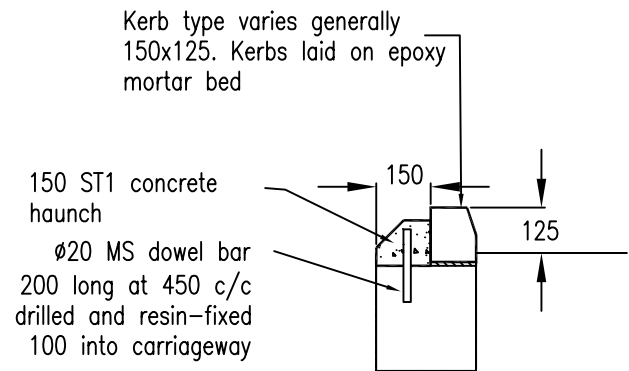
KERBS LAID ON EXISTING CONCRETE RACE OR CARRIAGEWAY
